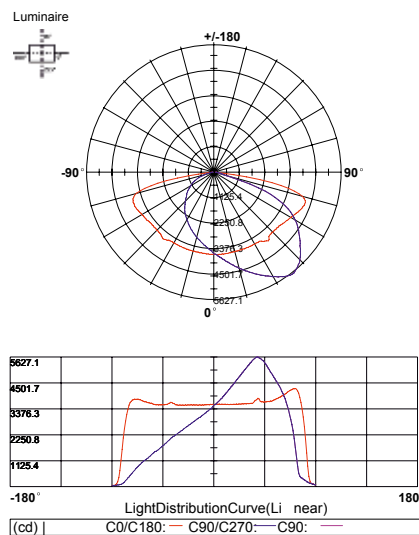
Light Distribution Curve [Unit:cd]
